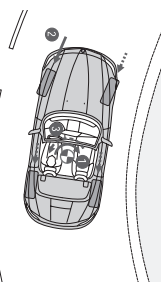
Cornering Brake Control (CBC) increases vehicle stability by proportioning the braking force while turning. When you brake in a turn, the pressure comes off the rear wheels, which (1) causes the vehicle to swerve inward (oversteer). Cornering Brake Control counteracts this action by asymmetrically adjusting brake pressure (2), creating stabilizing counter-torque (3) independently of the ABS system.
