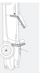
Z4 Roadster Rollover Protection System consists of two steel roll bars behind the headrests; they are connected with a highly stable chassis crossbeam. The system is completed by a bar of high-strength tubular steel integrated into the windshield frame for maximum safety.
